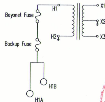
Connection Diagram
